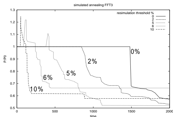
Figure 6. Plot of (\text{optimized power}) / (\text{initial power}) vs. time for simulated annealing algorithm on FFT3 application.
