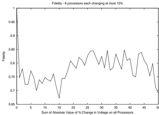
Figure 2. Plot of fidelity (equation 3) for six processor system vs. magnitude of voltage change on all processors
