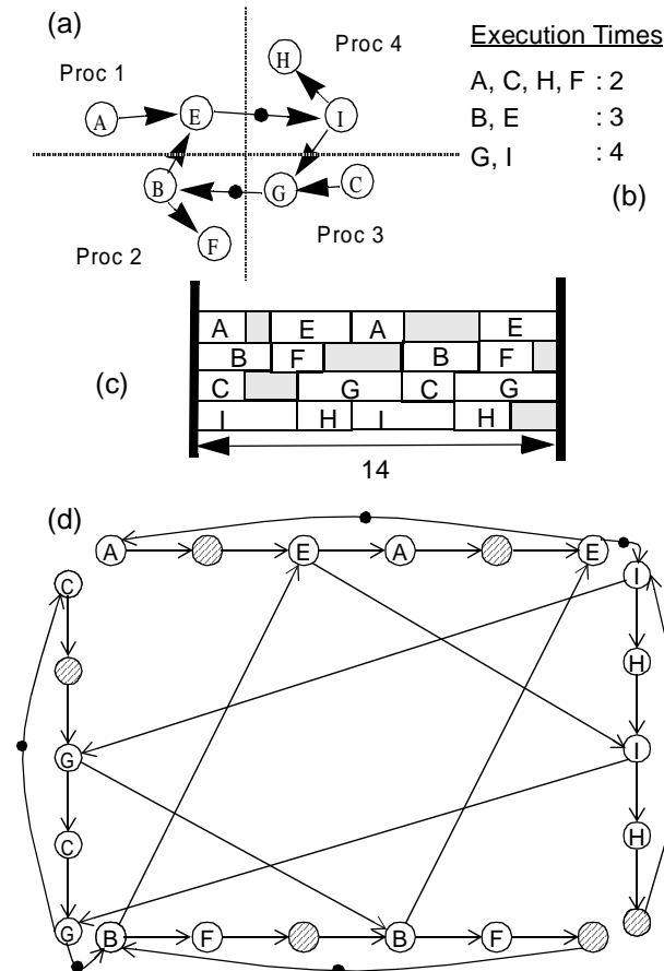
Figure 1. An illustration of the period graph model.
