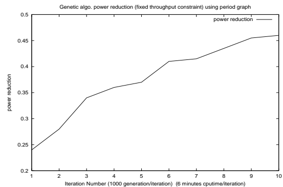
Figure 4. Plot of 1 - (\text{optimized power}) / (\text{initial power}) vs. genetic algorithm iteration using the period graph estimator.
