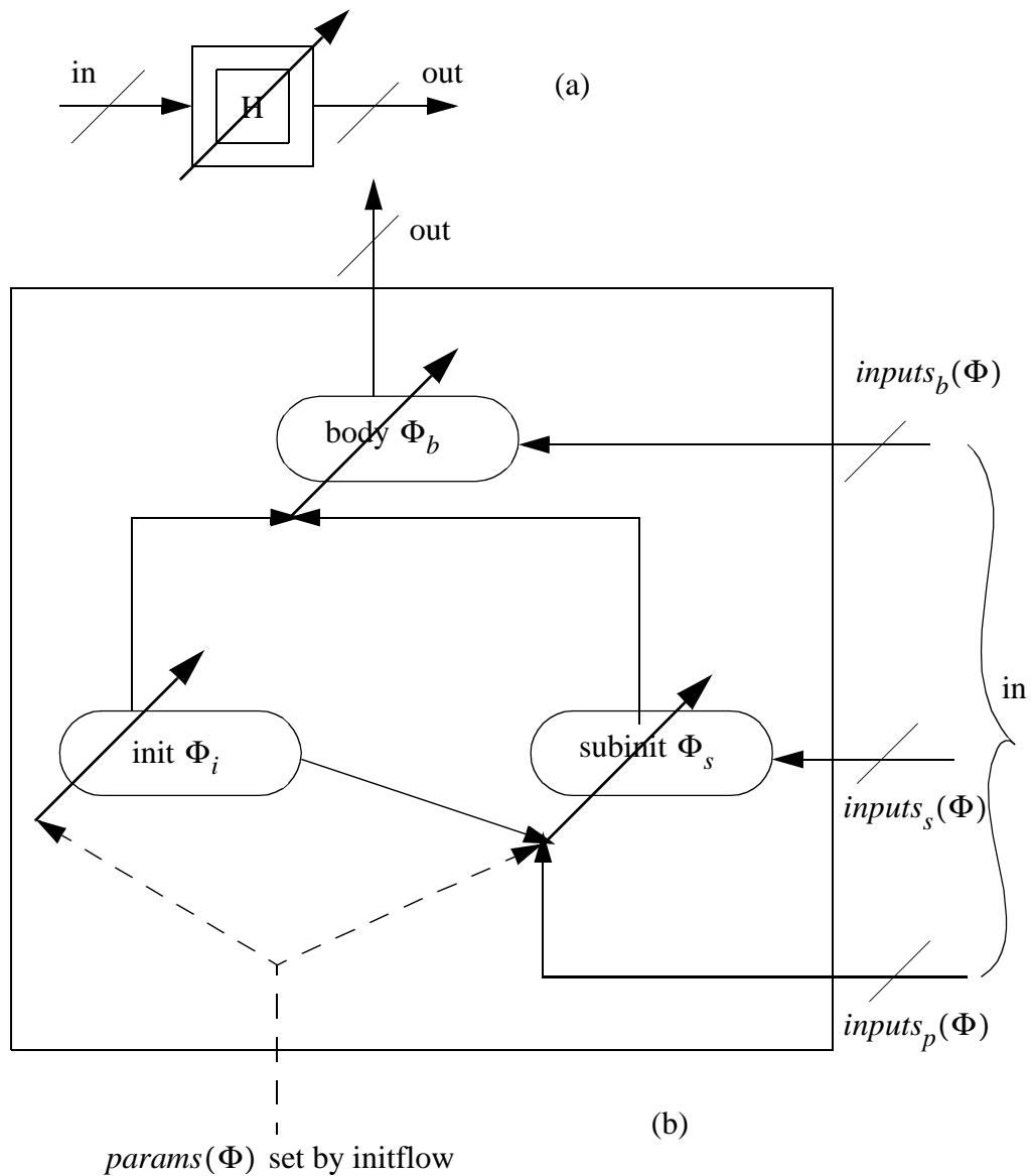
Figure 14. The operational structure of a PSDF specification. (a) shows a hierarchical PSDF actor H as it appears externally, and (b) shows the internals of the specification \Phi represented by H . A wide tip arrow on a block indicates the existence of parameters of that block that have to be configured externally. A slash on an input or output edge indicates a group of edges. Dataflow is denoted by bold lines, while initflow is denoted by dashed lines.
