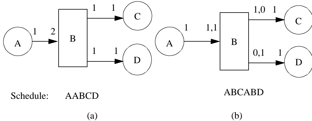
Figure 5. The cyclo-static dataflow model compared with synchronous dataflow. Actor B is a distributor actor. (a) SDF specification. (b) CDDF specification.
