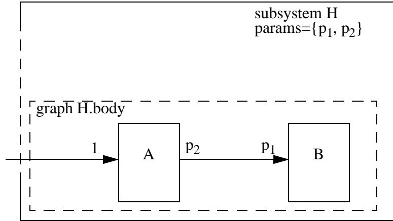
Figure 29. The body graph of a subsystem \Phi , where \Phi is represented by the hierarchical actor H . This example is used to demonstrate local synchrony verification issues in quasi-static scheduling. Different conclusions can be reached about the local synchrony of \Phi , depending on where (init graph or subinit graph) the parameters p_1 and p_2 are set.
