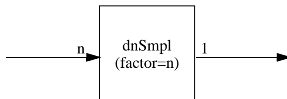
Figure 7. Downsampling by a variable factor in PSDF.
