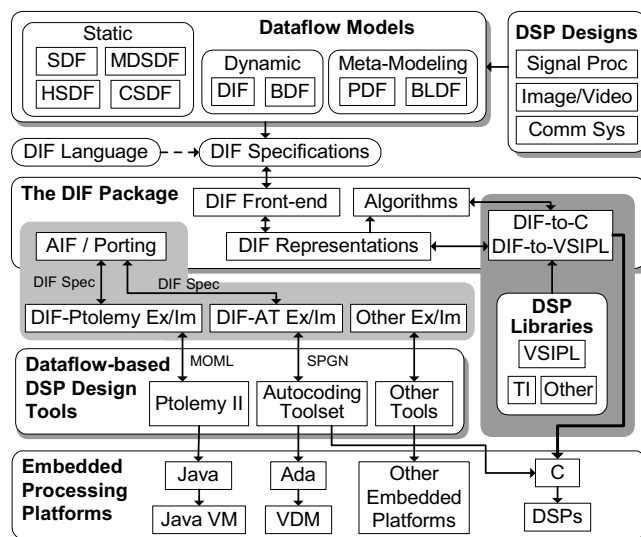
Figure 1: Methodology of using DIF.
